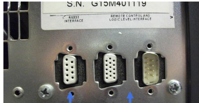
RS232 Interface
